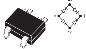
SMDIP CASE
